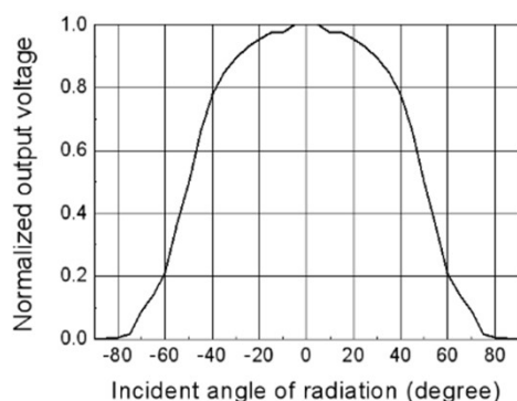
Optical characteristics
